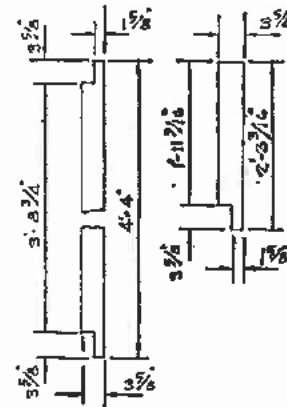
STIFFENER DETAILS
