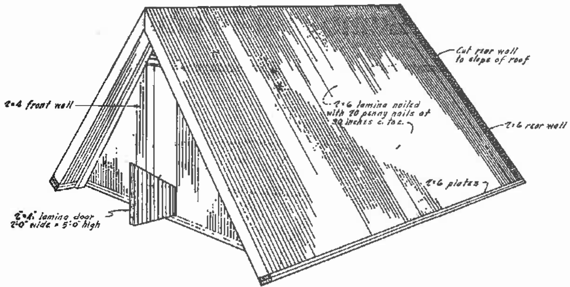
PERSPECTIVE VIEW
