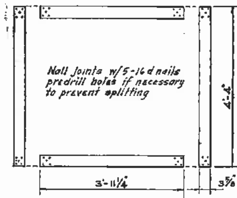
FRAME DETAIL
