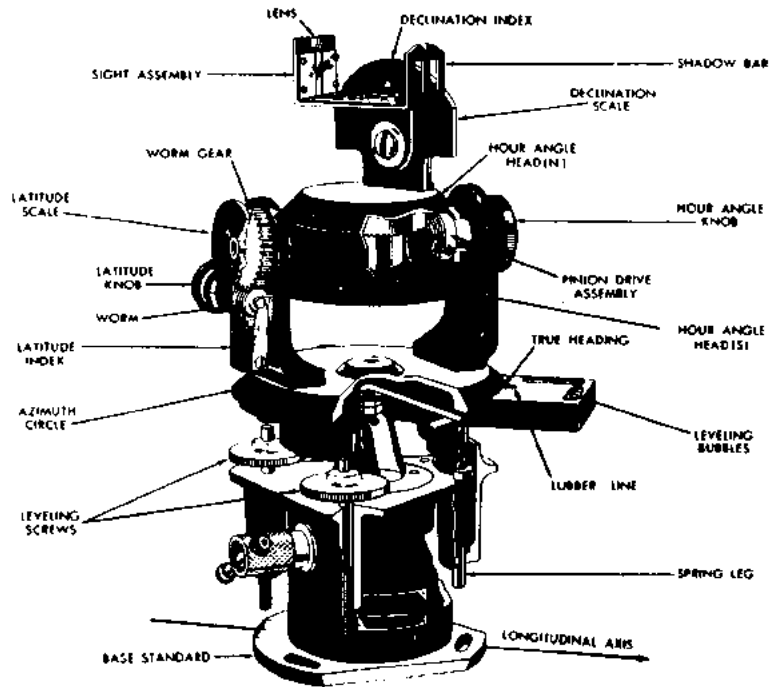
Figure C-1 Astro Compass
