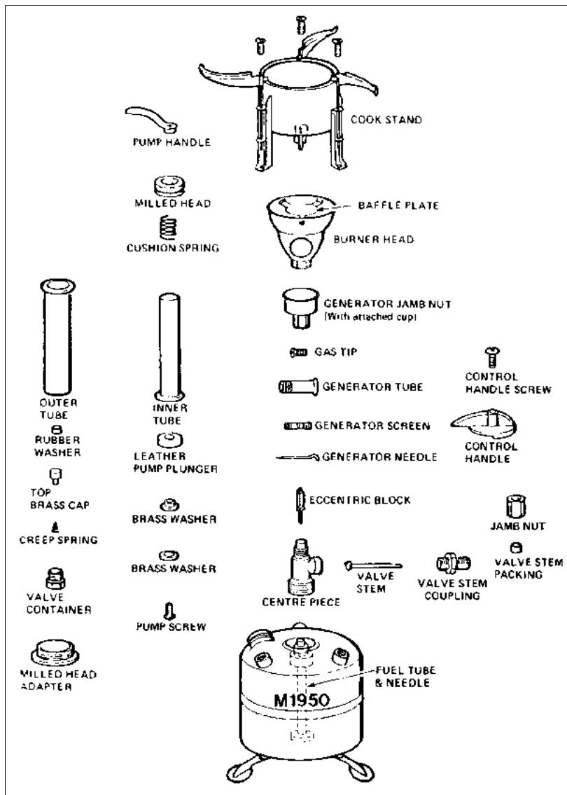
Figure 2-7A Stove M1950
