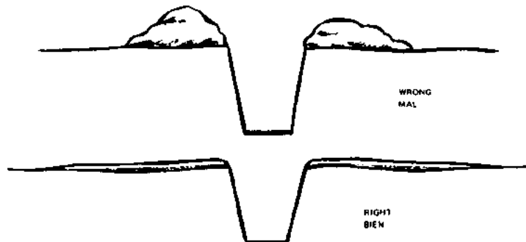
Figure 4-19 Snow Trench
