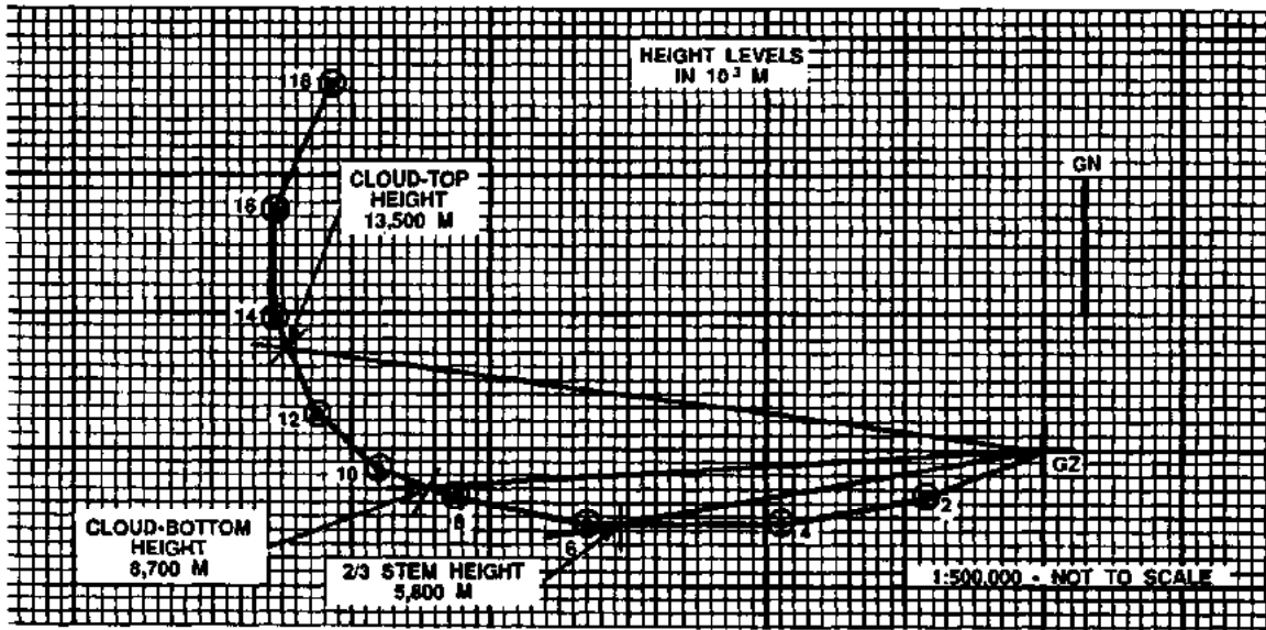
Figure 4-4. Initial determination of radial lines.
