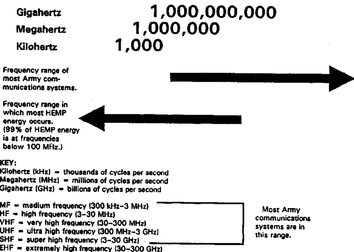
Figure C-5. Radio and EMP frequencies.
