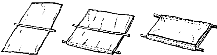
Figure B-21. Litter made with blanket and poles.
