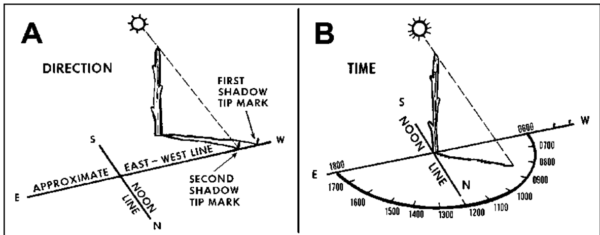
Figure II-1. Stick and Shadow Method
