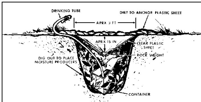
Figure VII-8. Solar Still
