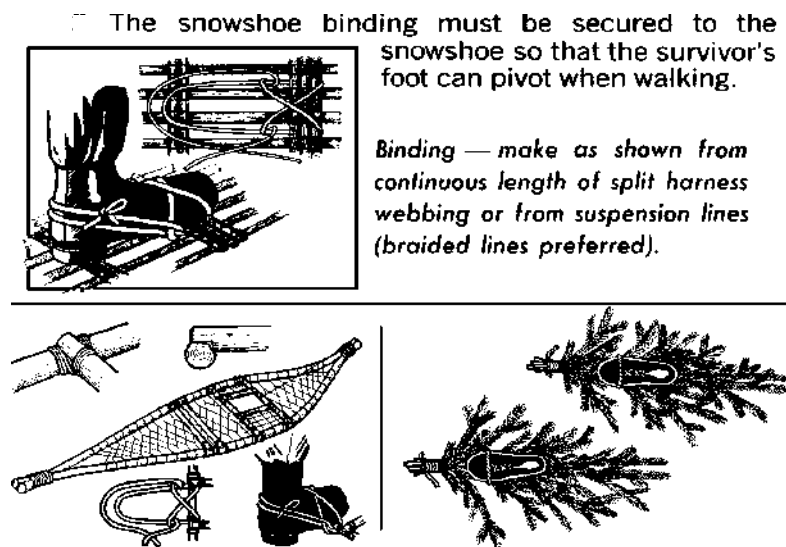
Figure II-10. Improvised Snowshoes
