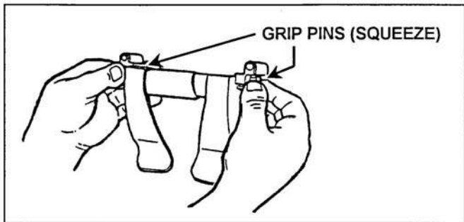
Figure 071-030-0011-10. Gripping of pins on feed throat assembly
