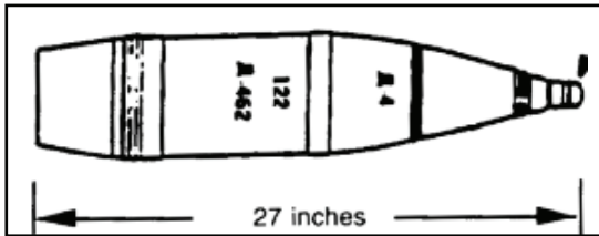
Figure 093-401-5040-4a. Projected projectile
