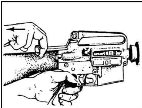
Figure 071-311-2027-5. Charging handle
