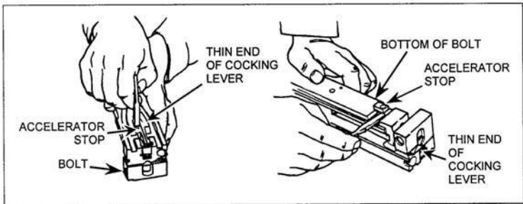
Figure 071-022-0001-13. Removal of the accelerator stop
