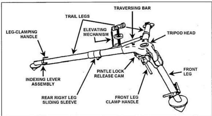
Figure 071-030-0011-2. M3 tripod
