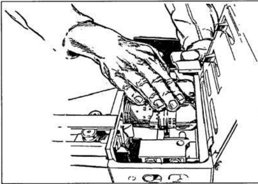
Figure 071-030-0005-2. Pushing round across feeder pawls
