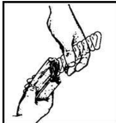
Figure 071-311-2025-42. Removing the magazine spring and the follower
