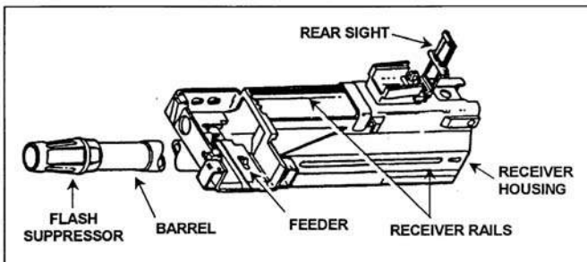
Figure 071-030-0001-15. Receiver assembly
