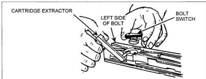
Figure 071-022-0001-9. Removal of the cartridge extractor and bolt
