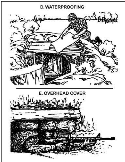
Figure 071-326-5703-5. Constructing overhead cover (continued)
