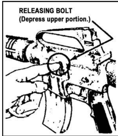
Figure 071-311-2027-7. Bolt catch
