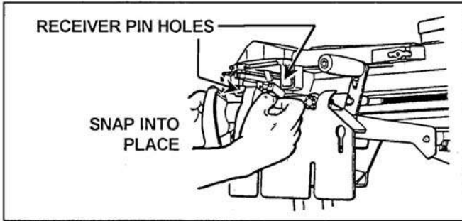
Figure 071-030-0011-11. Insertion of feed throat assembly
