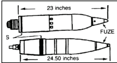
Figure 093-401-5040-5b. Mortars
