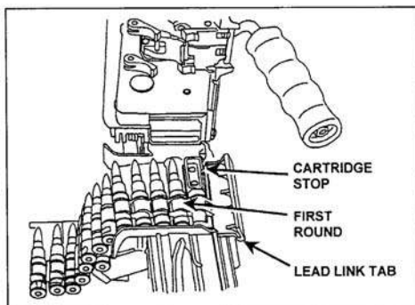
Figure 071-312-4027-4. Link belt in the feed tray
